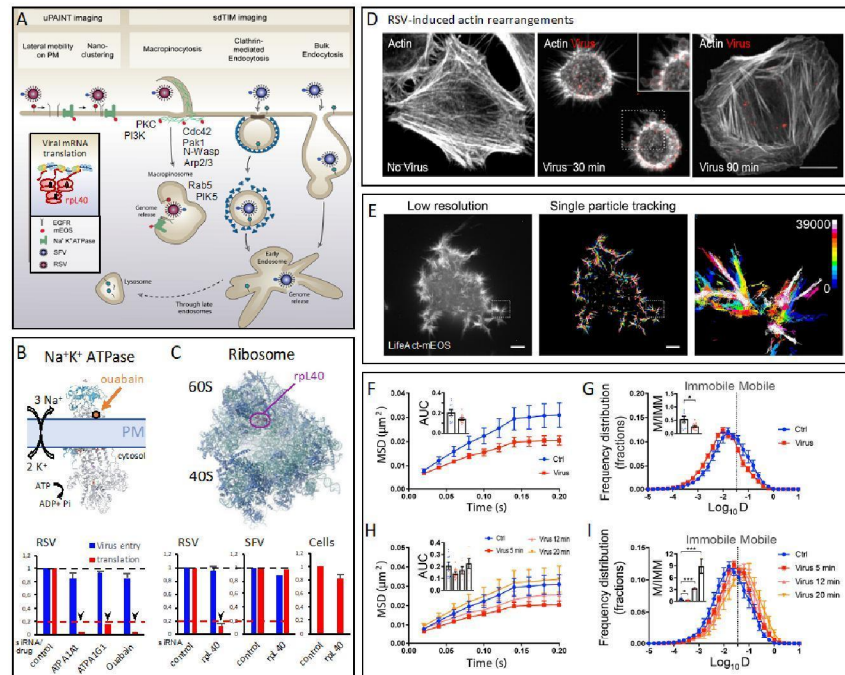
Figure 2. Identification of host regulators of RSV infection using single molecule imaging. A ) Schematic presentation of the single-molecule imaging approaches to study virus mobility and nanoclustering on the PM (uPAINT) and upon internalization (sdTIM). B-C ) Validation of top hits identified by genome-wide siRNA screen for RSV. Depletion or inhibition of Na + K + ATPase subunit components ( B ) inhibits a post-entry step of RSV infection (arrowheads), whereas depletion of ribosomal component rpl40 ( C ) inhibits RSV translation. D ) RSV (red spots) induces dramatic, time-dependent changes in the cellular actin cytoskeleton. E ) Single molecule tracking (LifeAct-mEos) of actin dynamics during virus infection. Scale bar is 5 μm and the color-coding refers to the time-frame of image acquisition. F ) Quantification of single molecule mobility (mean square displacement, MSD; μm 2 s -1 ) of LifeAct-mEos in RSV-infected (red line) or non-infected (blue line) cells. The area under the MSD curve (AUC; in arbitrary units [a.u.]) is shown in the inset. G ) Significant decrease in the mobility of LifeAct-mEos upon virus infection indicates a higher binding rate of the construct to F-actin, which most likely is the result of induced actin polymerization. H-I ) Changes in actin dynamics upon RSV infection are transient, showing a trend of initial decrease and subsequent return of the actin mobility to control levels based on (H) MSD, (I) Log 10 D and M/IMM quantifications. Statistical analyses of independent experiments were performed using the Student's t test and the statistical significance is indicated as * p <0.05, *** p <0.001. Error bars are ±SEM.
